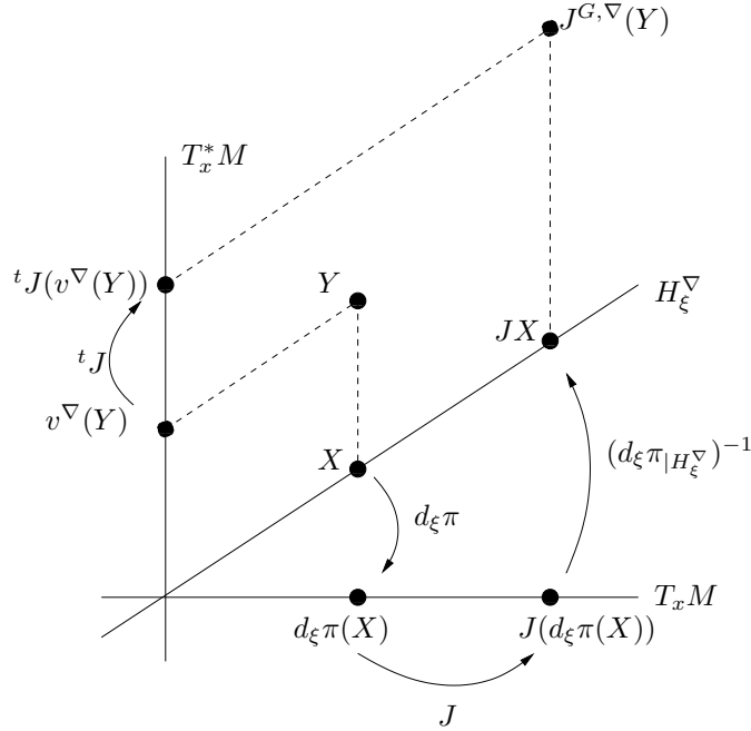
Figure 1. Construction of the generalized horizontal lift J^{G,\nabla} .
